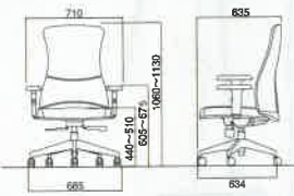
座面寸法: W540×D515
